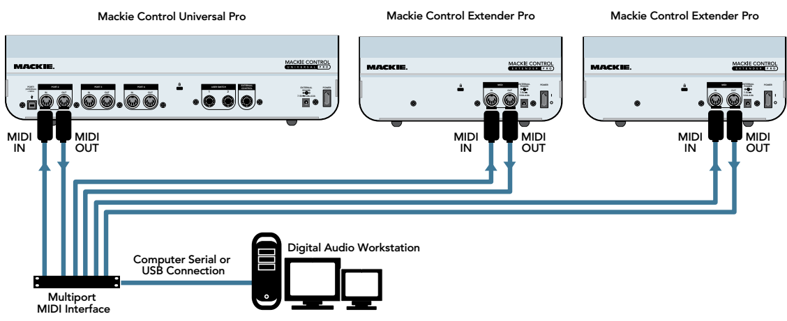
Hookup 2: MIDI
