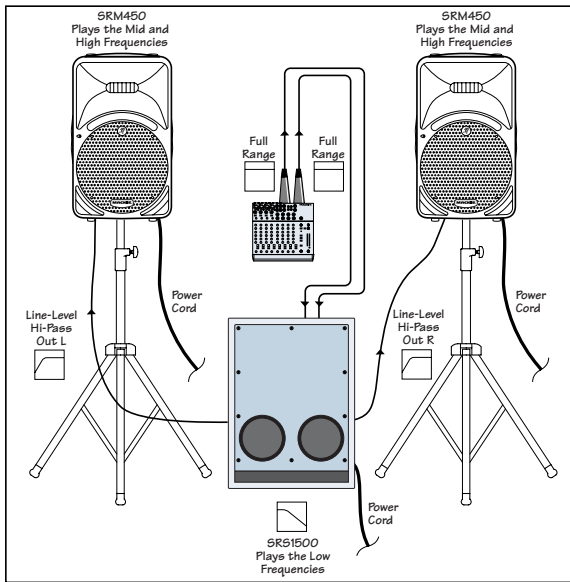
1 SRS1500 WITH 2 SRM450s
