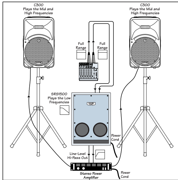
1 SRS1500 WITH STEREO AMPLIFIER AND 2 C300s
