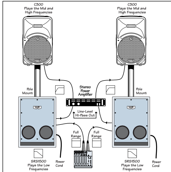
2 SRS1500s WITH STEREO AMPLIFIER AND 2 C300s
