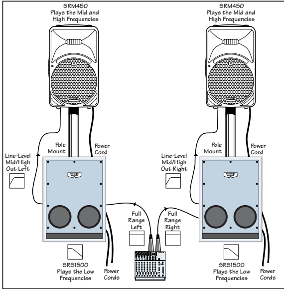
2 SRS1500s WITH 2 SRM450s
