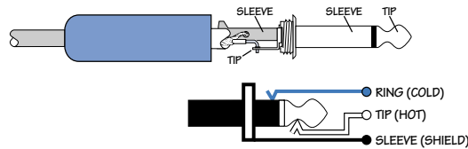
Unbalanced 1/4" TS Plug
